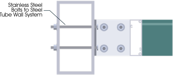
Typical Sunshade to Steel Support Installation
